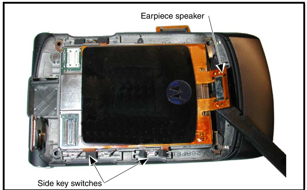
Figure 16. Earpiece Speaker and Side Key Switch Flex Cables
