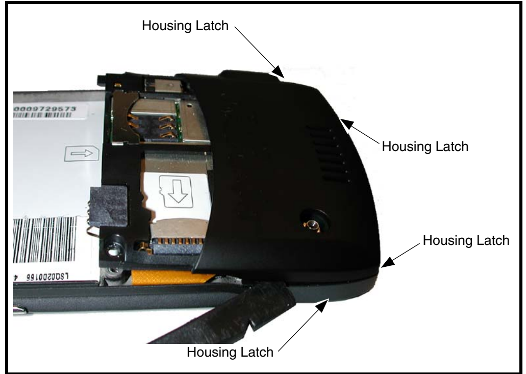
Figure 6. Removing the Rear Housing Latches
