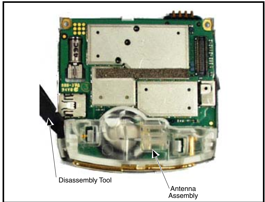
Figure 9. Removing the Antenna Assembly
