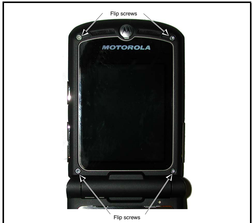
Figure 11. Removing the Flip Assembly Screws
